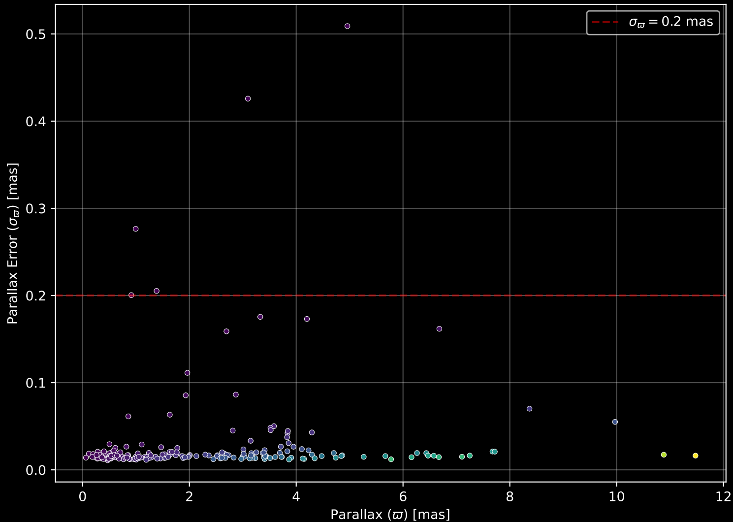
APOGEE DR17 Field: [193+27_MGA] Parallax Quality (n= 202)
