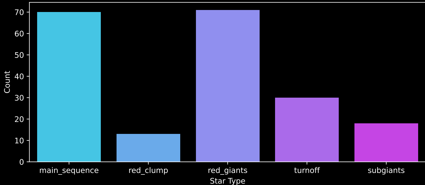
APOGEE DR17 Field: [193+27_MGA] Count plot of Star Type
