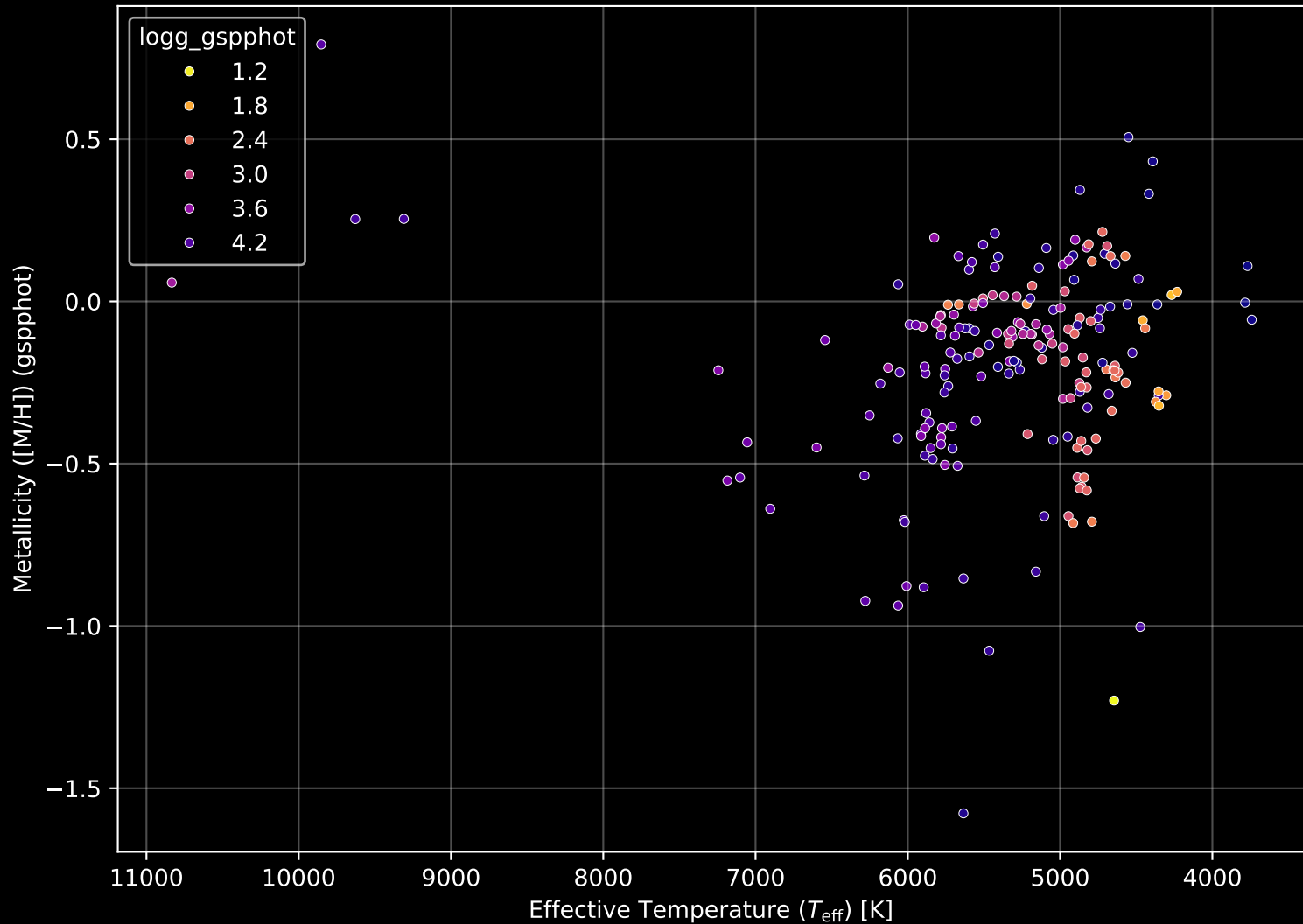
APOGEE DR17 Field: [193+27_MGA] Stellar Population Parameters (n= 202)
