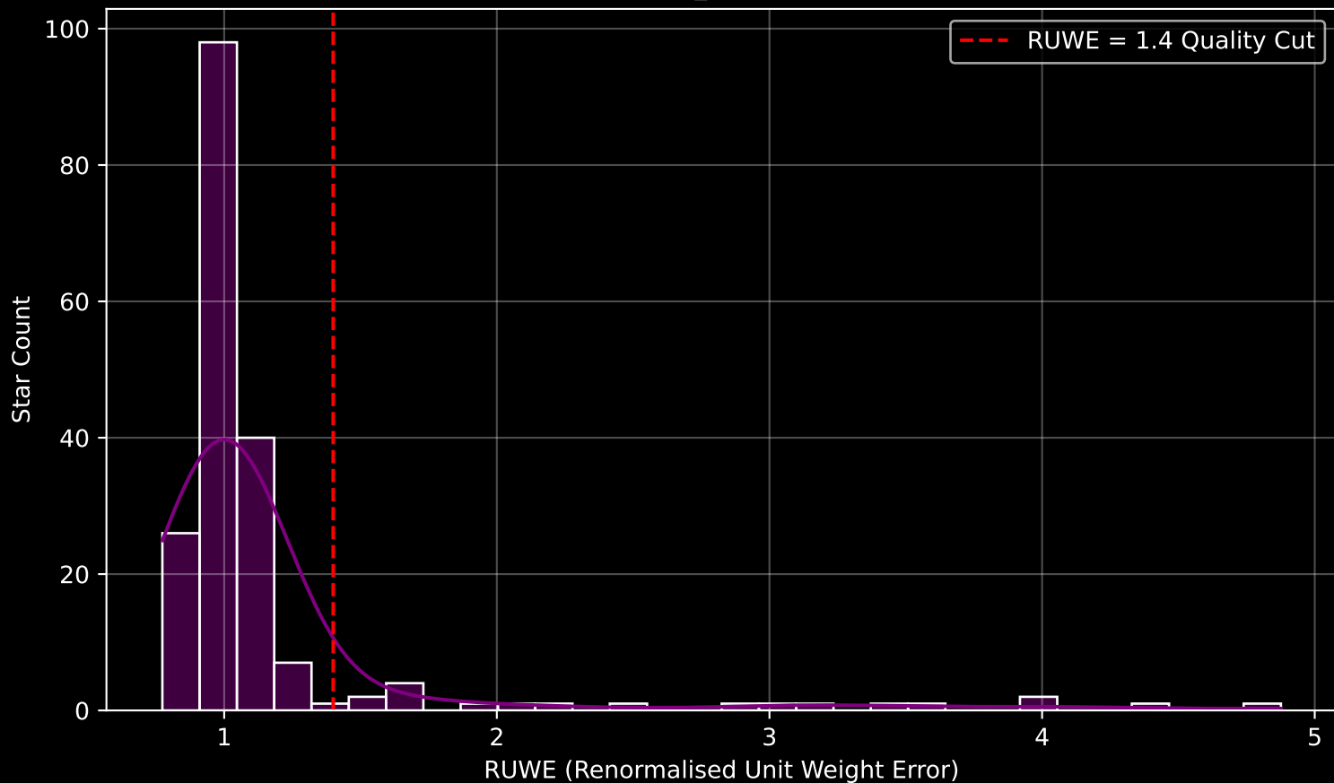
GAPOGEE DR17 Field [193+27_MGA] RUWE Distribution (n= 191)
