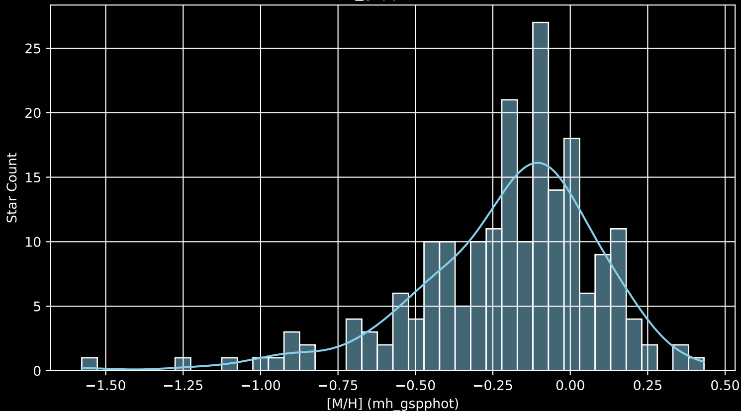
APOGEE DR17 Field: [193+27_MGA [M/H] (mh_gspphot) (n= 200)
