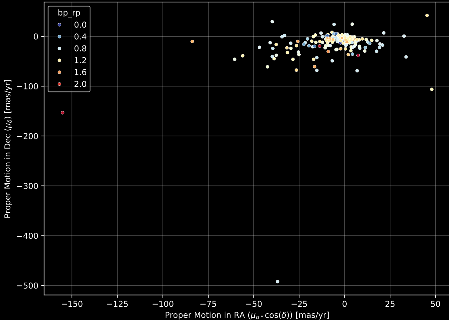
APOGEE DR17 Field: [193+27_MGA] Proper Motion Diagram (n= 202)
